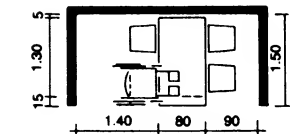
④ Dining area for two/four people
